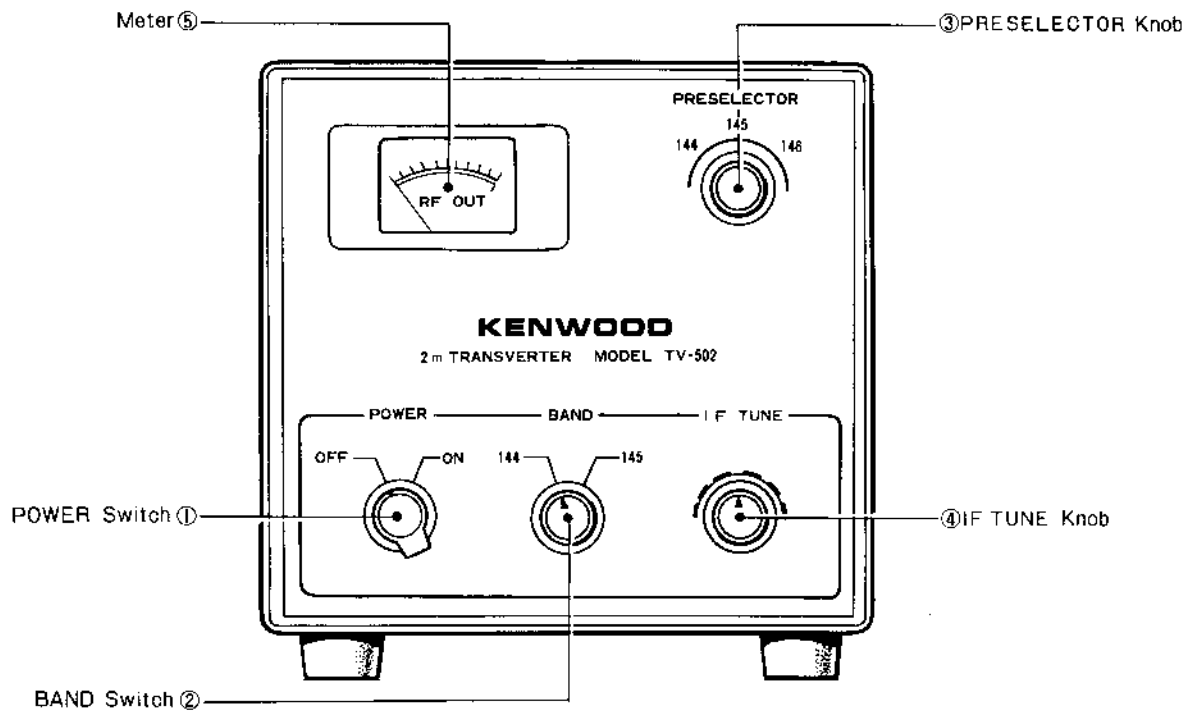
Fig. 2 Front Panel
