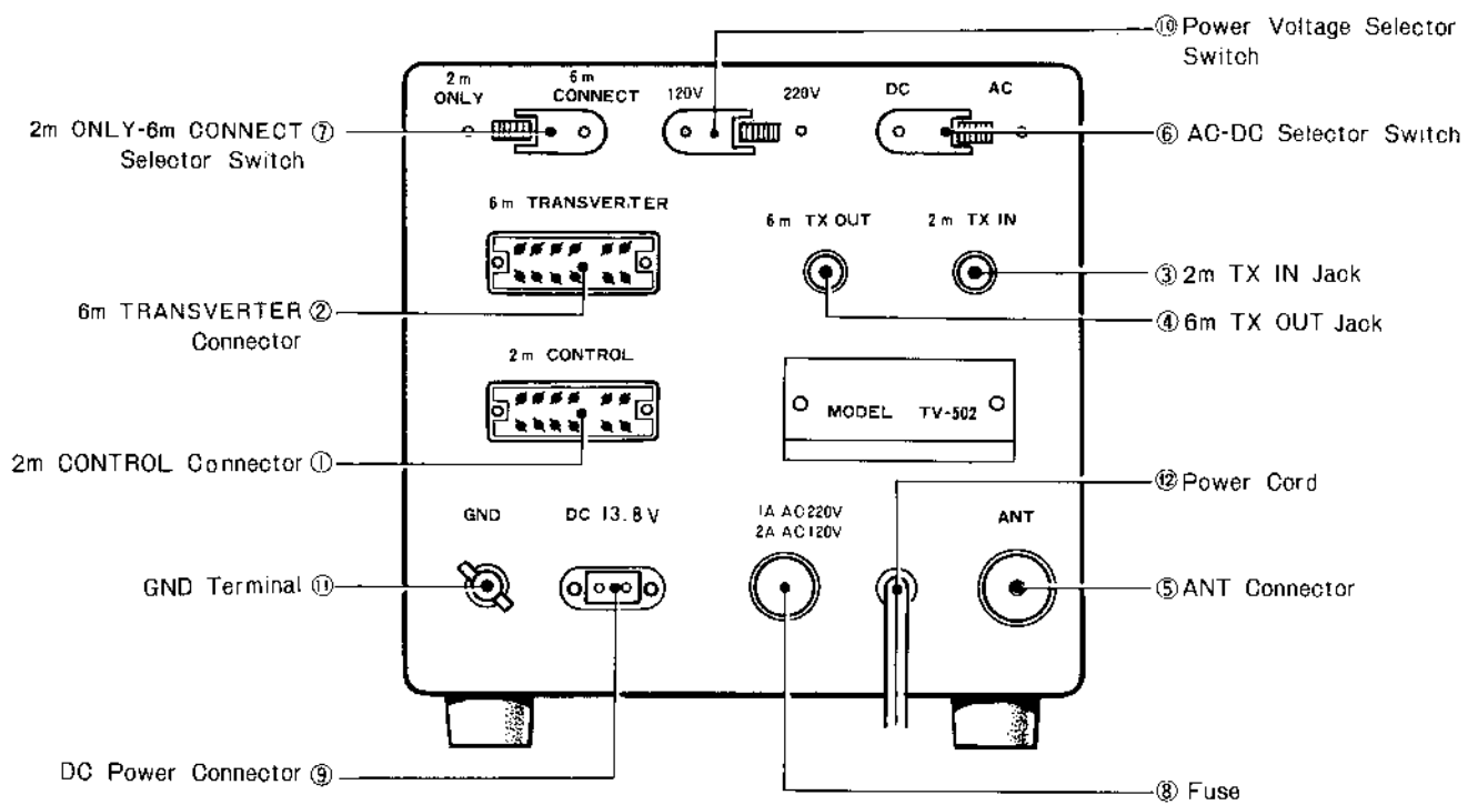
Fig. 3 Rear Panel
